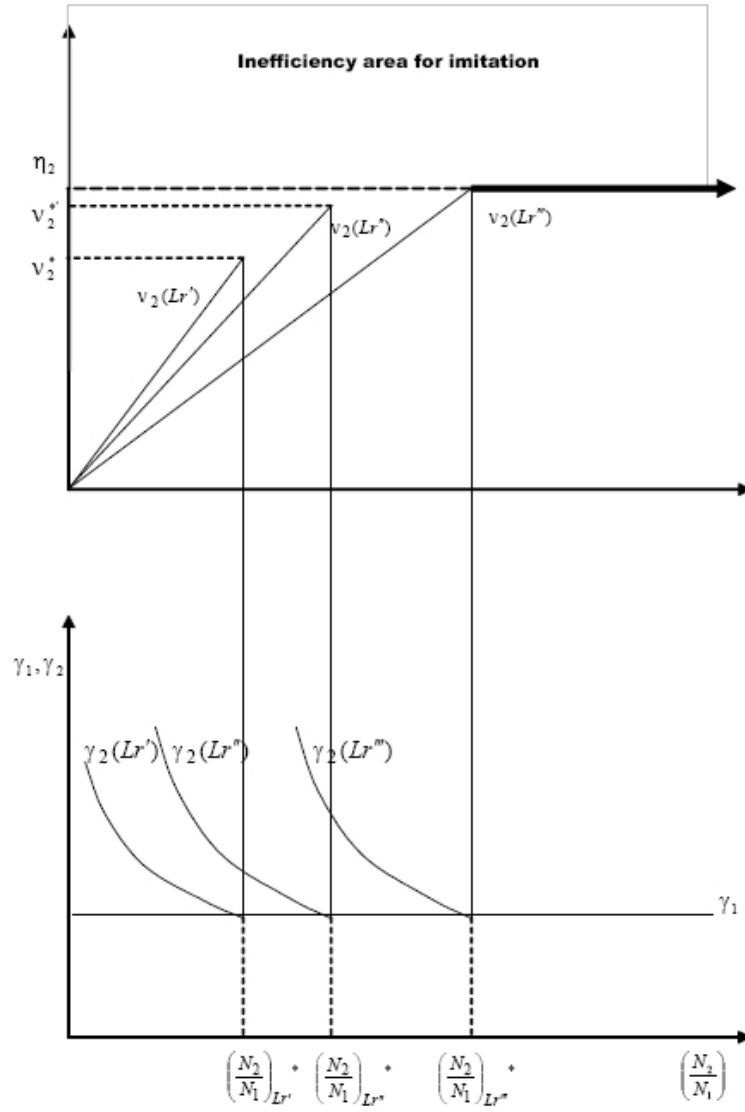
Figure 1: Transitional dynamics
